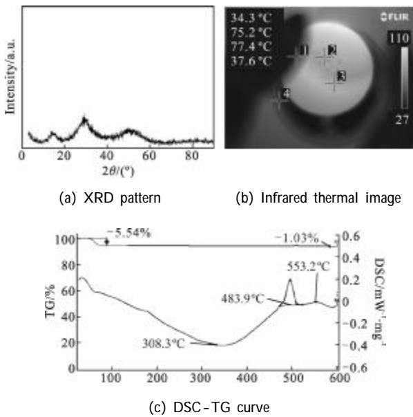
图 4 \text{Ge}_{28}\text{Sb}_{12}\text{Se}_{60} 玻璃的 XRD 谱线、热成像图和 DSC-TG 曲线 Fig.4 XRD pattern, infrared thermal image and DSC-TG curve of \text{Ge}_{28}\text{Sb}_{12}\text{Se}_{60} glasses
