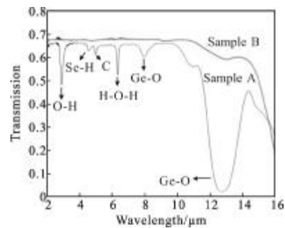
图 5 \text{Ge}_{28}\text{Sb}_{12}\text{Se}_{60} 玻璃试样中远红外透过光谱 Fig.5 IR transmission spectra of \text{Ge}_{28}\text{Sb}_{12}\text{Se}_{60} glasses
