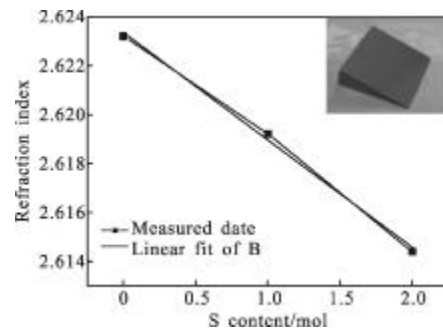
图 6 \text{Ge}_{28}\text{Sb}_{12}\text{Se}_{60-x}\text{S}_x ( x=0, 1, 2 ) 玻璃在 4 \mu\text{m} 处的折射率(内图为测试用楔形样) Fig.6 Refraction indices of \text{Ge}_{28}\text{Sb}_{12}\text{Se}_{60-x}\text{S}_x ( x=0, 1, 2 ) glasses at 4 \mu\text{m} wavelength(the inset is a picture of cuneiform sample)
