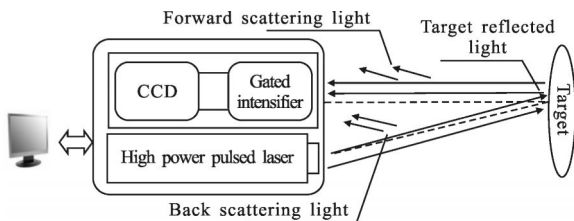
图 1 水下距离选通成像技术原理图 Fig.1 Underwater range-gated imaging technology
