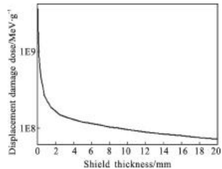
Fig.4 Shielding effect of displacement damage dose for a five years mission at sun-synchronous orbit of 900 km
