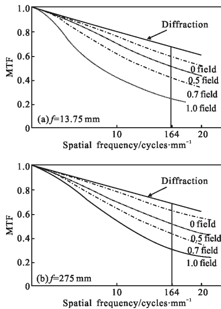
图 6 20×中波红外相机镜头传递函数曲线 Fig.6 MTF of MWIR camera lens with 20× ratio
