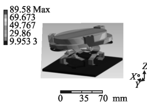
(b) 二阶模态-偏转 (b) 2nd mode-tilt
