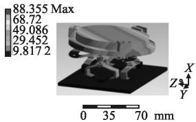
(c) 三阶模态-偏转 (c) 3rd mode-tilt
