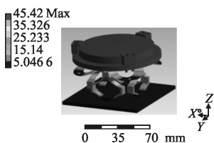
(a) 一阶模态-轴向平移 (a) 1st mode-axial translation
