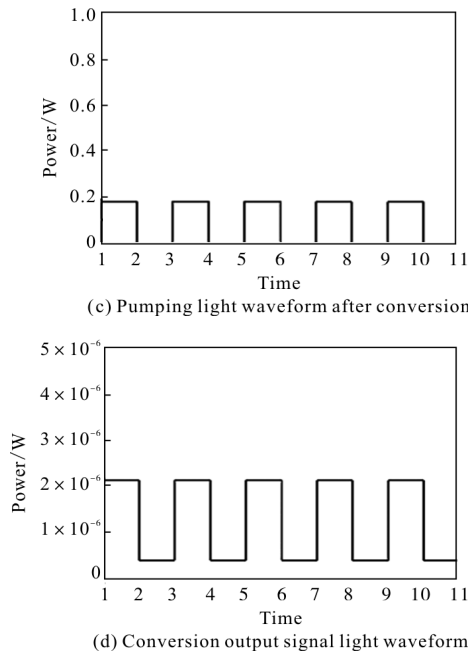
Fig.2 Conversion process waveform
