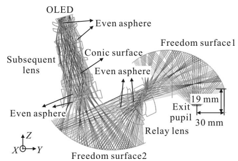
图 4 双自由曲面大视场头盔显示光学系统 Fig.4 Wide field-of-view head-mounted display optical system with double freeform surfaces
