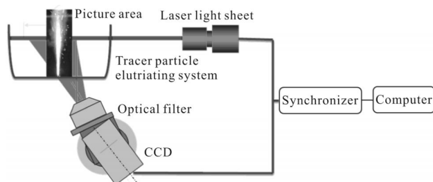
Fig.1 Schematic diagram of the PIV system
