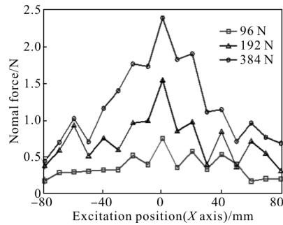
图 12 不同激励源位置的裂纹面法向接触力 Fig.12 Normal contact force of crack faces with different excitation positions
