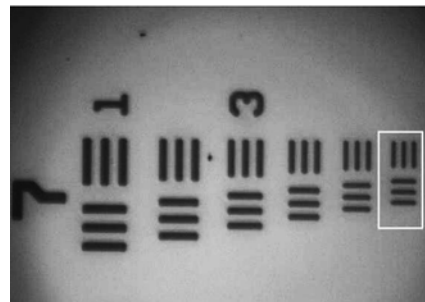
图 8 同轴监测系统的分辨率评价 Fig.8 Resolution evaluation of coaxial monitoring system
