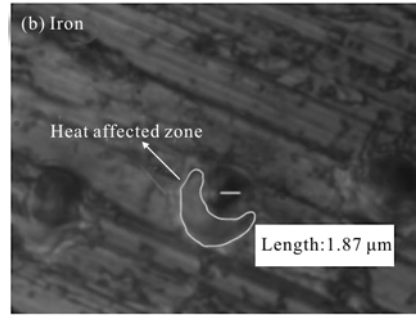
图 7 基于 Al 纯样(a)和 Fe 纯样(b)的激光探针极限分辨率 Fig.7 Ultimate resolution of laser probe based on Al pure sample (a) and Fe pure sample (b)
