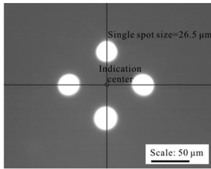
图 9 同轴监测画面中的指示光图样与尺寸 Fig.9 Indicator light patterns and dimensions in coaxial monitoring screen
