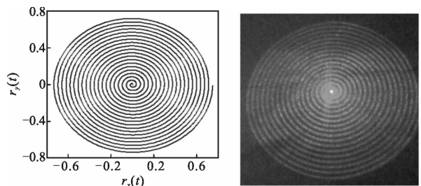
(e) 螺旋线指令信号 (f) 螺旋线指令信号轨迹扫描图 (e) Command signal of helical line (f) Track scanning of command signal of helical line
