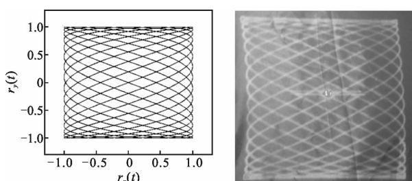
(a) 李萨如图指令信号 (b) 李萨如图扫描轨迹 (a) Command signal of Lissajous pattern (b) Trajectory diagram of Lissajous pattern
