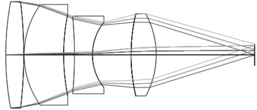
Fig.2 Initial structure of imaging objective lens of imaging system
