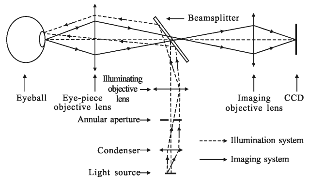
Fig.1 Schematic diagram of system design
