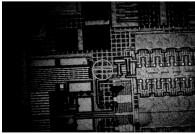
(a) 敏感位置 1: 脉冲激光能量为 13 nJ (a) Sensitive area 1#: pulse laser energy is 13 nJ
