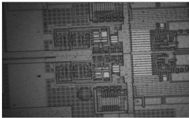
(b) 敏感位置 2: 脉冲激光能量 6 nJ (b) Sensitive area 2#: pulse laser energy is 6 nJ
