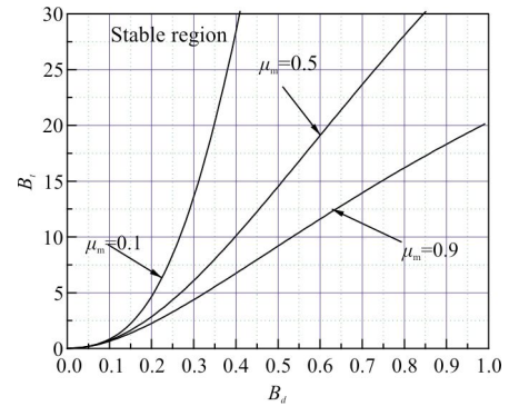
Fig.3 Stable region with \mu_m at 0.1, 0.5, and 0.9
