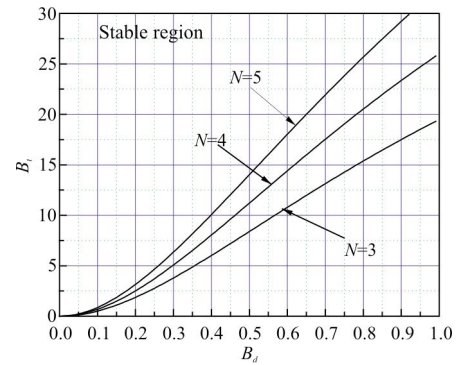
Fig.2 Stable region with N at 3, 4, and 5
