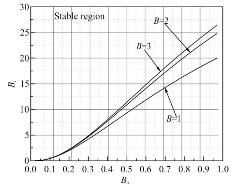
Fig.4 Stable region with B at 1, 2, 3
