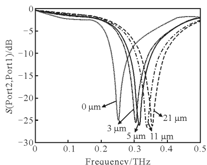
(b) 距离 d 对微带带阻滤波结构的影响的 S_{21} 参数 (b) S_{21} parameter for effect of GaAs sample with different distances on the band stop filter
