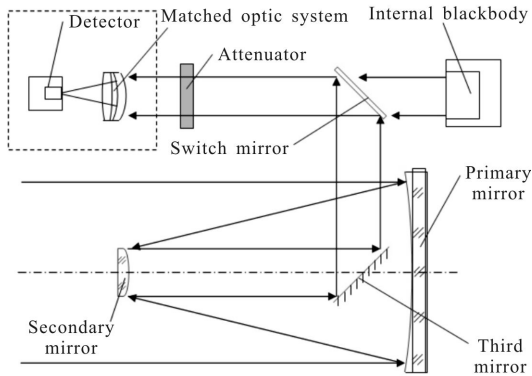
图 2 大口径光学系统及标定示意图 Fig.2 Diagram of large aperture optical system and calibration
