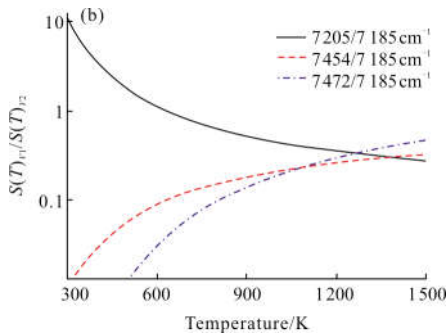
图 3 不同谱线强度(a)和谱线强度比值(b)随温度的变化 Fig.3 Different linestrengthes (a) and the ratio of linestrength versus temperature
