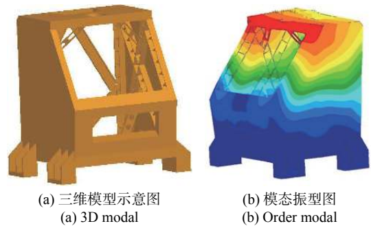
图 3 优化后主承力三维模型及模态振型图 Fig.3 3D modal and order modal of main frame after optimization
