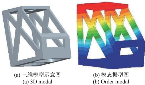
图 2 优化前主承力三维模型及模态振型图 Fig.2 3D modal and order modal of main frame before optimization
