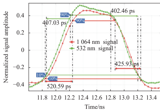
(c) 脉冲宽度 2 ns 的信号波形 (c) Signal waveform with pulse width 2 ns
