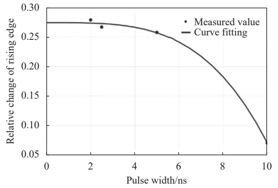
(a) 信号上升沿相对变化量的拟合结果 (a) The fitting result of the relative change along the rising edge of the signal
