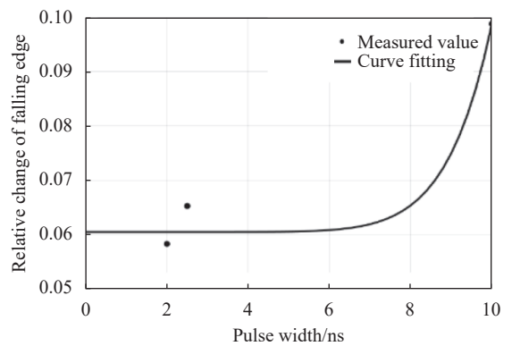
(b) 信号下降沿相对变化量的拟合结果 (b) The fitting of the relative variation along the falling edge of the signal
